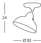
731.10.104 Deckenleuchte/ ceiling lamp 1 Ip., E27, 75 W/ LED E27
