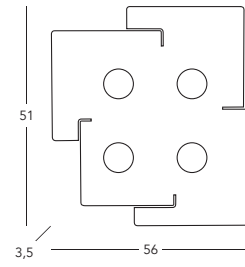
■ A1337.14.1.W Deckenleuchte/ceiling lamp 4 lp., incl. LED GX53, 7 W 2240 lm, 2700 K
