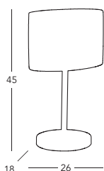
■ 1264.70.6 Tischleuchte / table lamp vernickelt / nickel plated 💡 1 lp., E27, 60 W / LED E27
